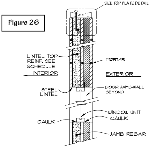
Figure 26 LINTEL DETAIL - 8"
