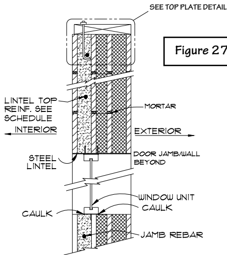
Figure 27 LINTEL DETAIL - 12"
