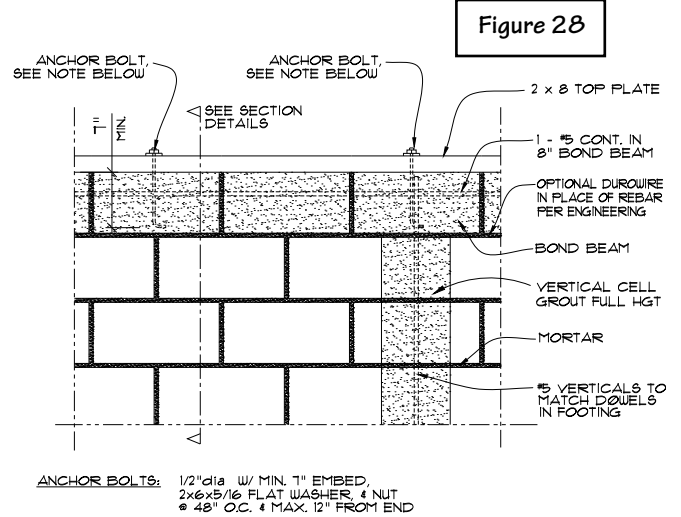
Figure 28 TOP PLATE DETAIL
