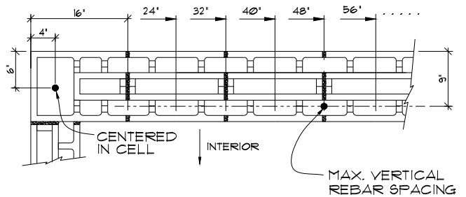
STANDARD WALL - 12"
