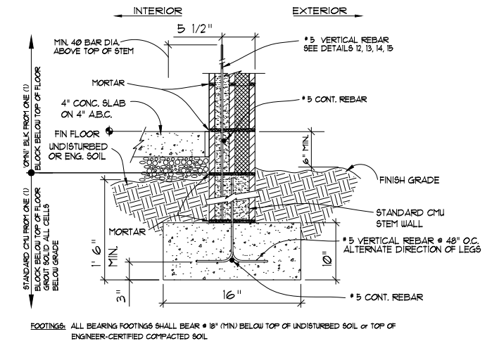
OPTION B - BLOCK STEM
