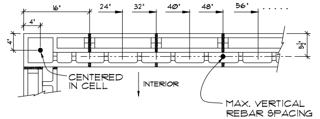
STANDARD WALL - 8"
