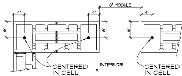
WINDOW / DOOR OPENINGS - 12"
