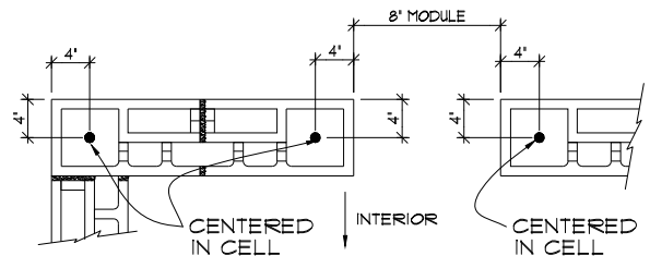
WINDOW / DOOR OPENINGS - 8"
