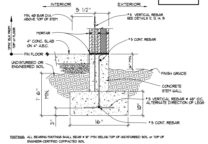
OPTION A - CONCRETE STEM
