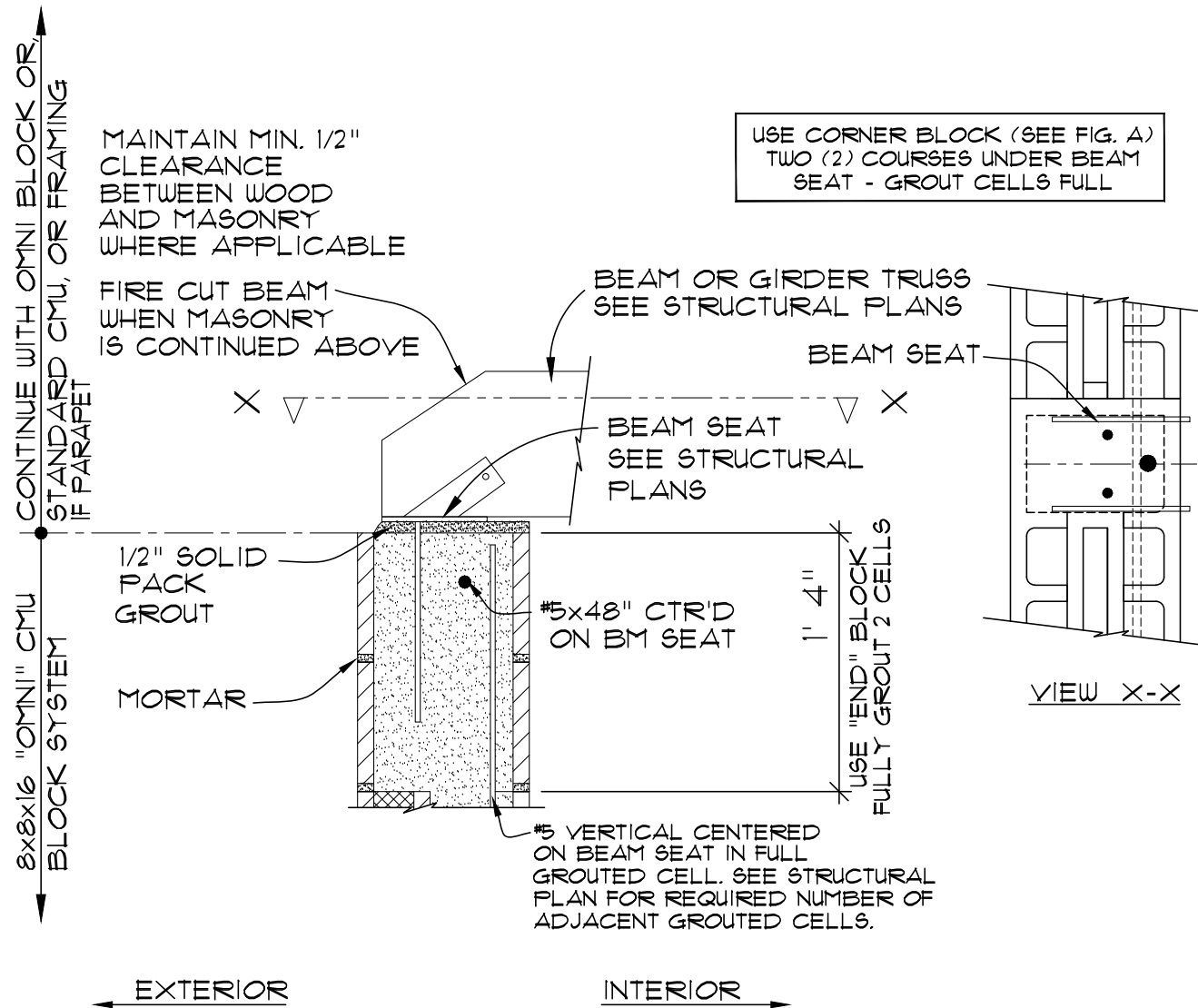
6 BEAM OR TRUSS @ CMU
