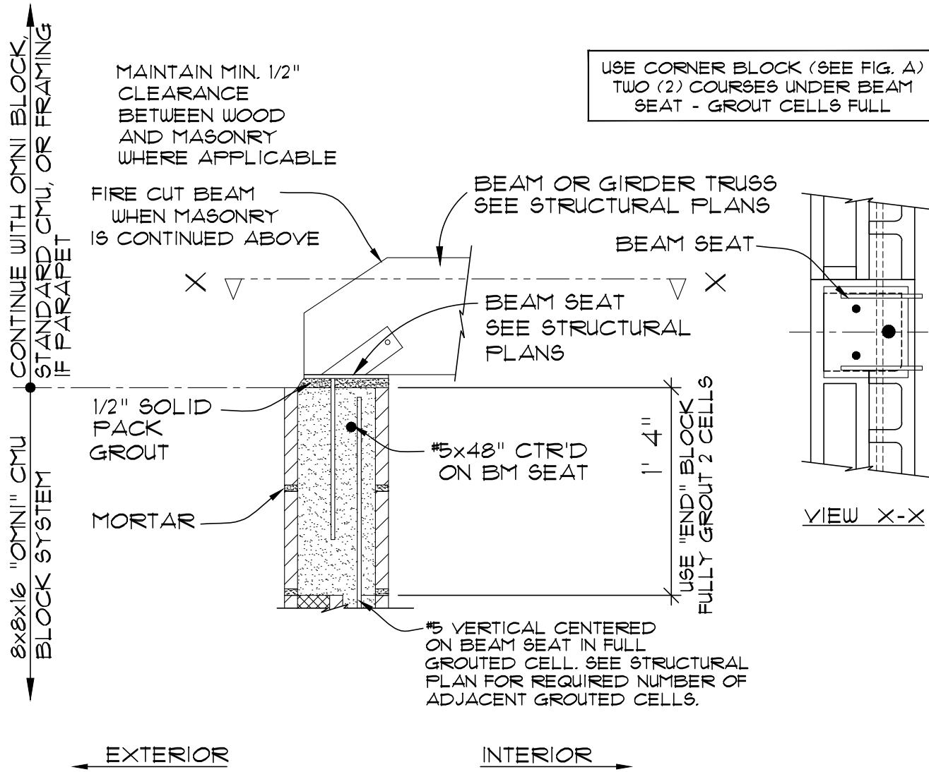
6 BEAM OR TRUSS @ CMU
